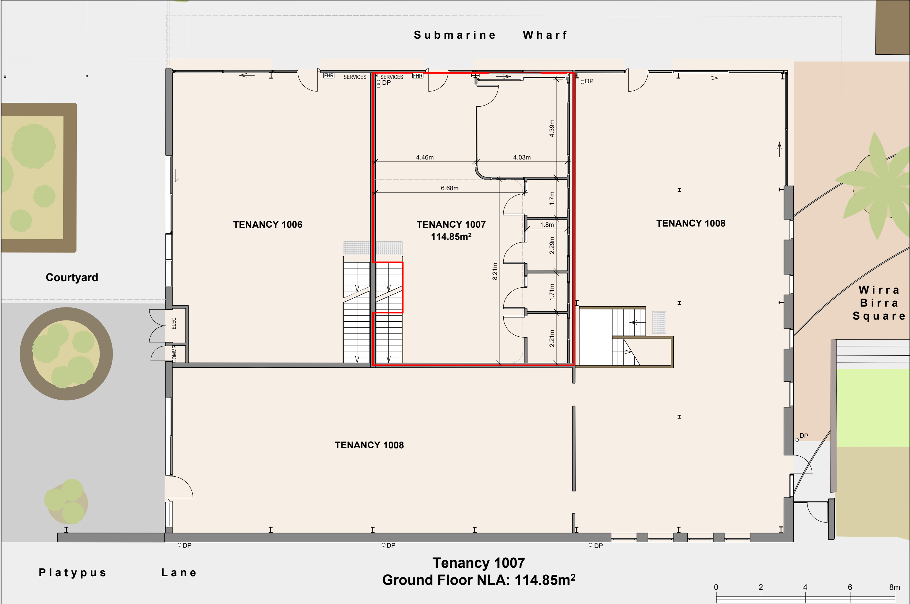
Tenancy 1007 - Ground Floor, Lease Plan
