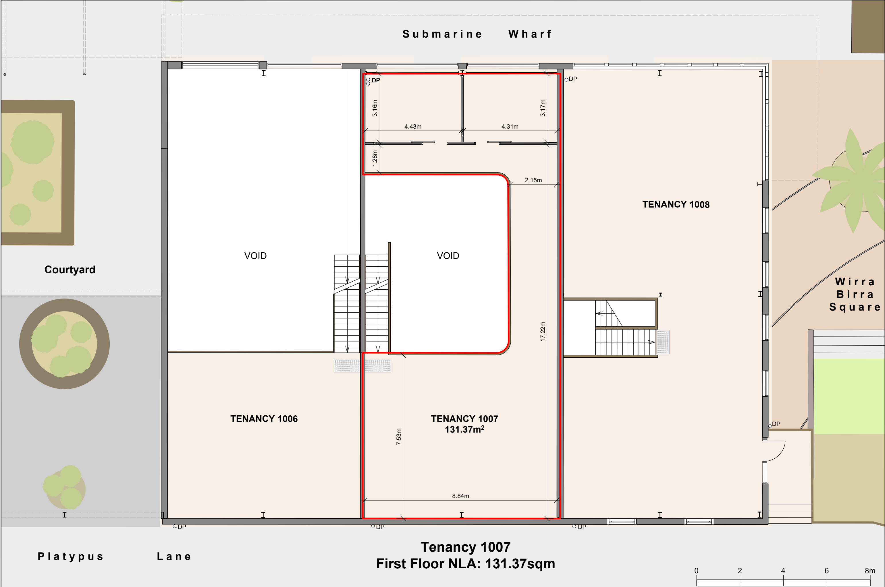
Tenancy 1007 - First Floor, Lease Plan
